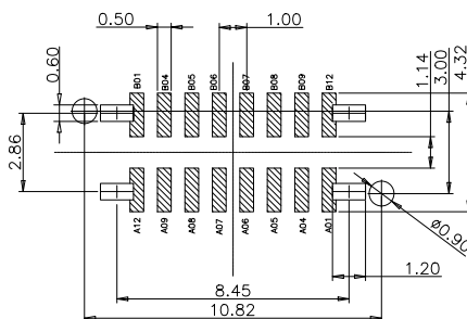
RECOMMENDED P.C.B. LAYOUT (俯视图) TOLERANCE UNSPECIFIED ±0.05mm
