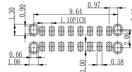
RECOMMENDED P.C.B. LAYOUT TOLERANCE UNSPECIFIED \pm 0.05\text{mm}
