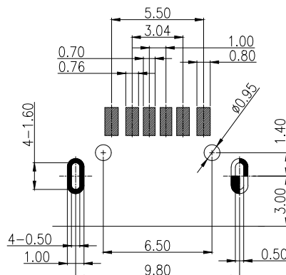
Recommended P.C.B. Layout Unspecified tolerance: \pm 0.05 (Top view)
